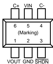
S9 Package (TSOT-23-6)
