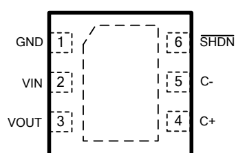
D7 Package (TDFN- 6) (2x2mm)
