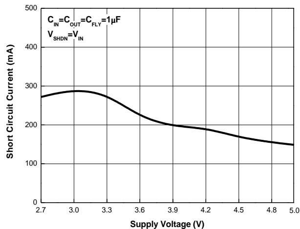
Figure 9. Short Circuit Current vs. Supply Voltage
