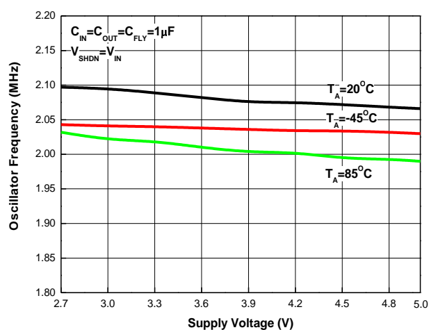
Figure 7. Oscillator Frequency vs. Supply Voltage
