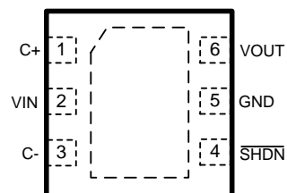
D7 Package (TDFN- 6) (2x2mm)
