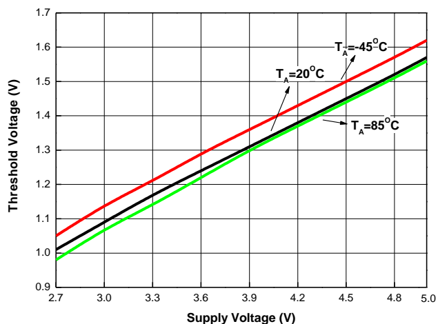
Figure 8. VSHDN Threshold Voltage vs. Supply Voltage
